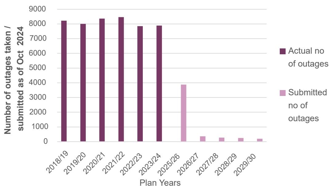
Figure 12: Number of outages taken / in plan
