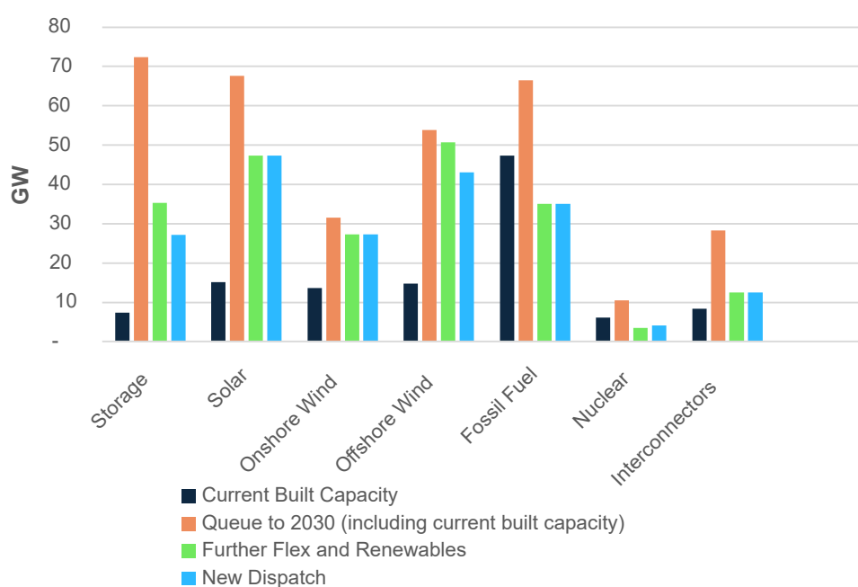
Figure 13: Current connections queue against clean power pathways by technology (GW)
