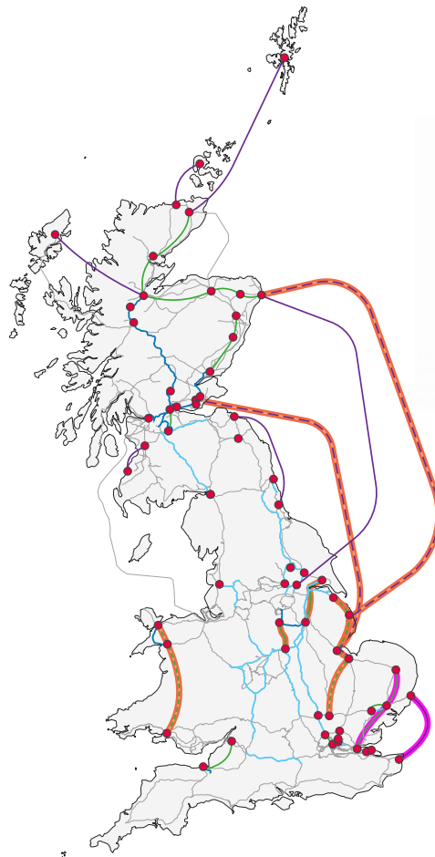
Figure 11: Map of 2030 transmission network reinforcements for a clean power system
