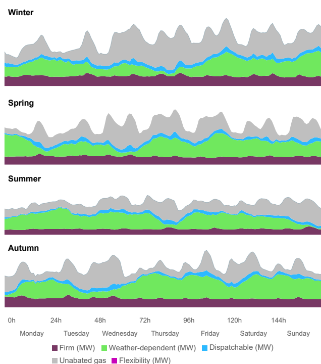
Figure 16: Modelled 7-day hourly generation profiles for 2023
