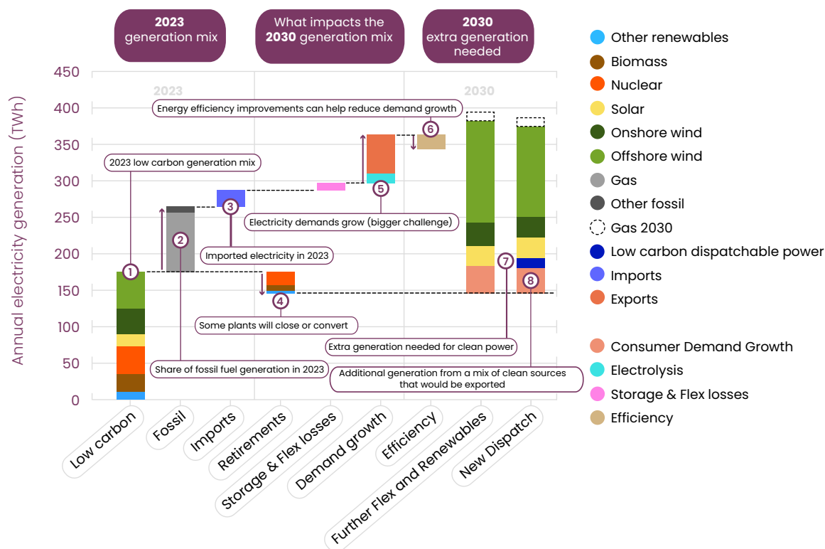
Figure 6: Increase in electricity supply for 2030
